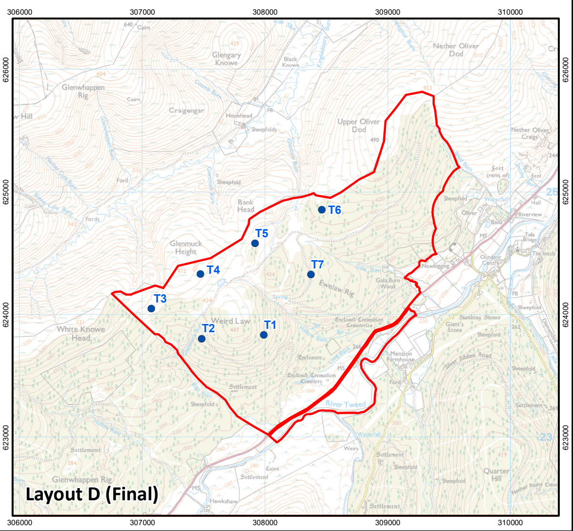
Figure 2.3 Wind Turbine Location Design Evolution Oliver Forest Wind Farm Environmental Impact Assessment Report
