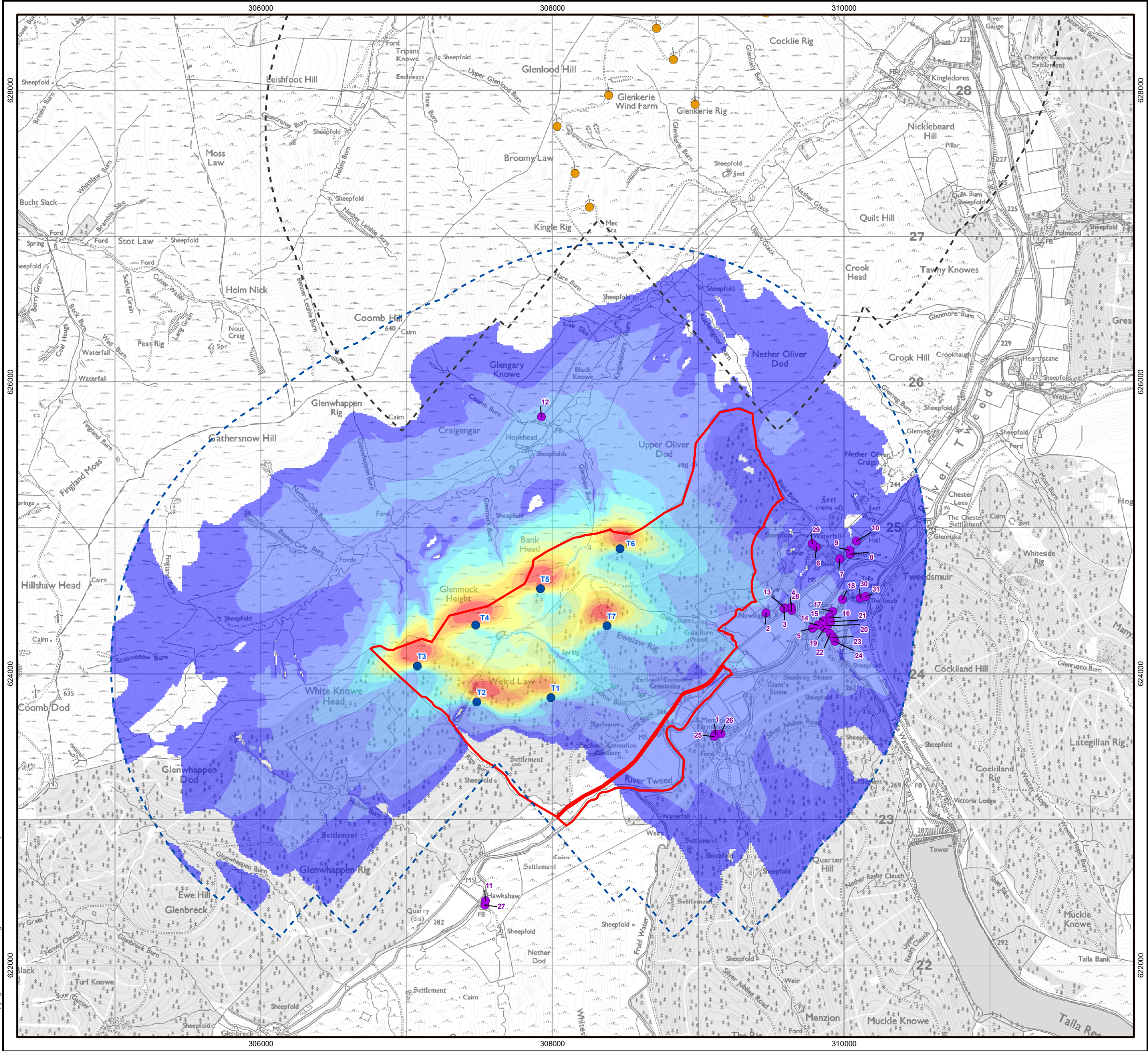
Figure 17.2 Shadow Flicker Results Oliver Forest Wind Farm Environmental Impact Assessment Report
