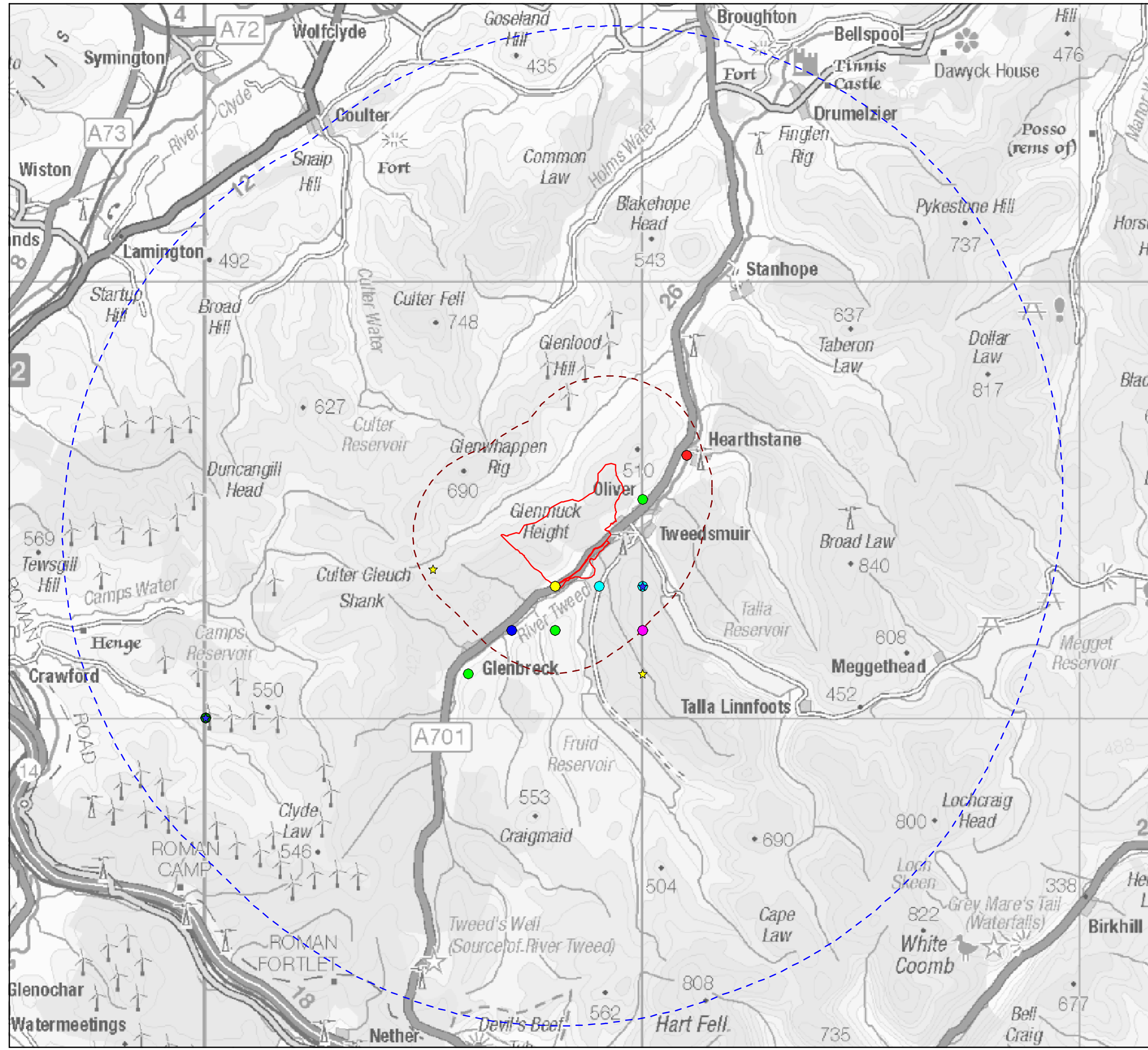
Figure 8.4 Desk Study Records - 'Invasive' Non-Native Species Oliver Forest Wind Farm Environmental Impact Assessment Report
