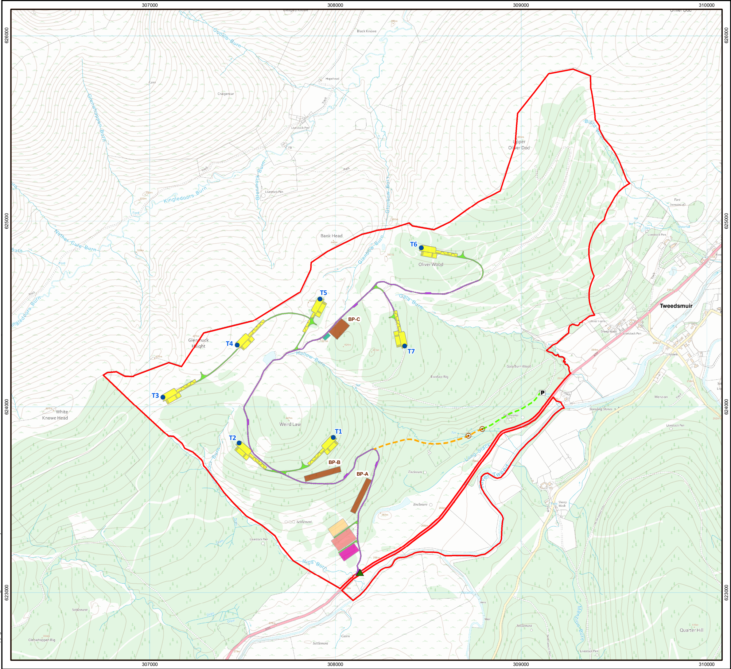
Figure 3.2 Site Layout Oliver Forest Wind Farm Environmental Impact Assessment Report
