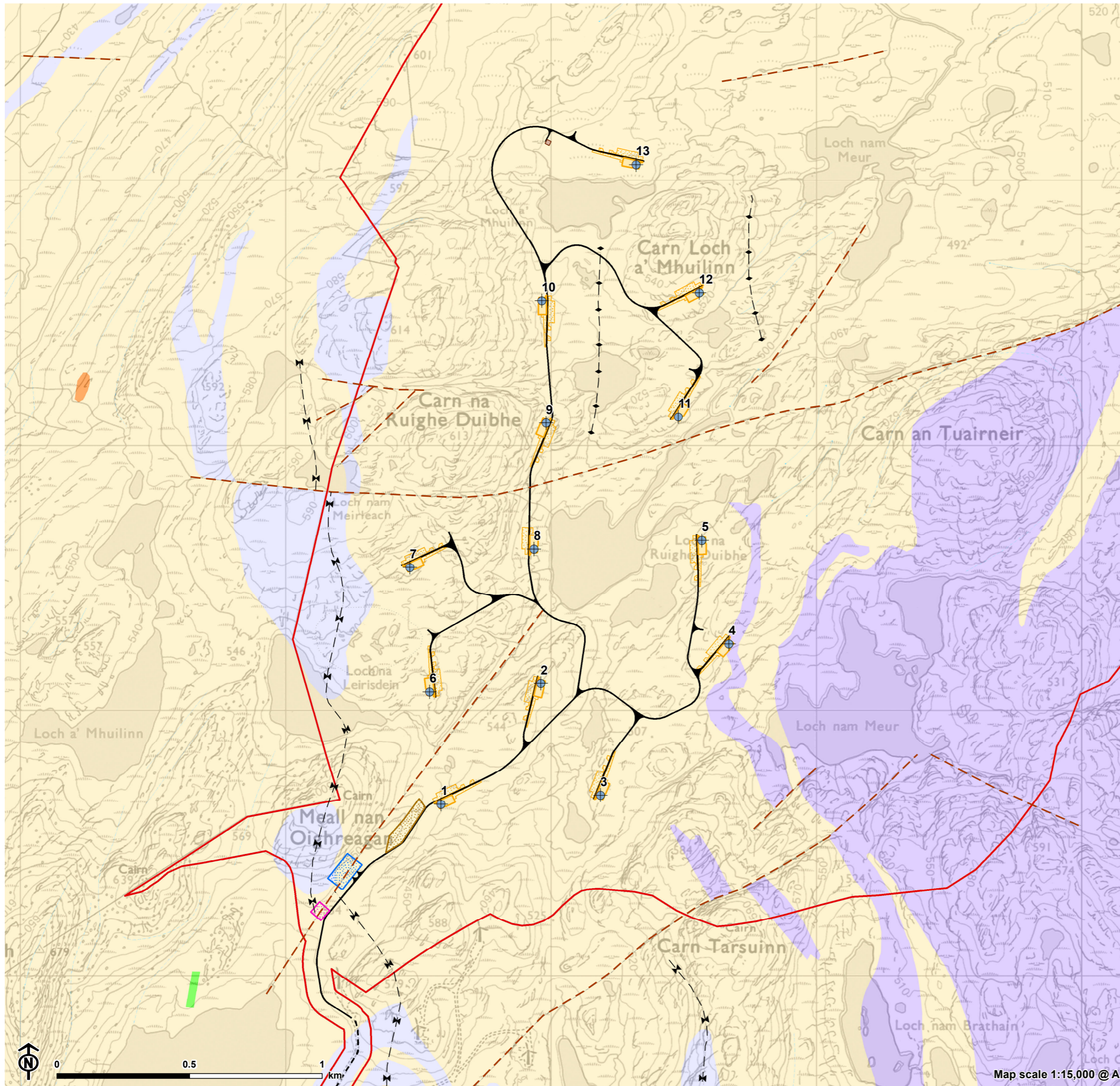
Figure 7.5: Bedrock Geology
