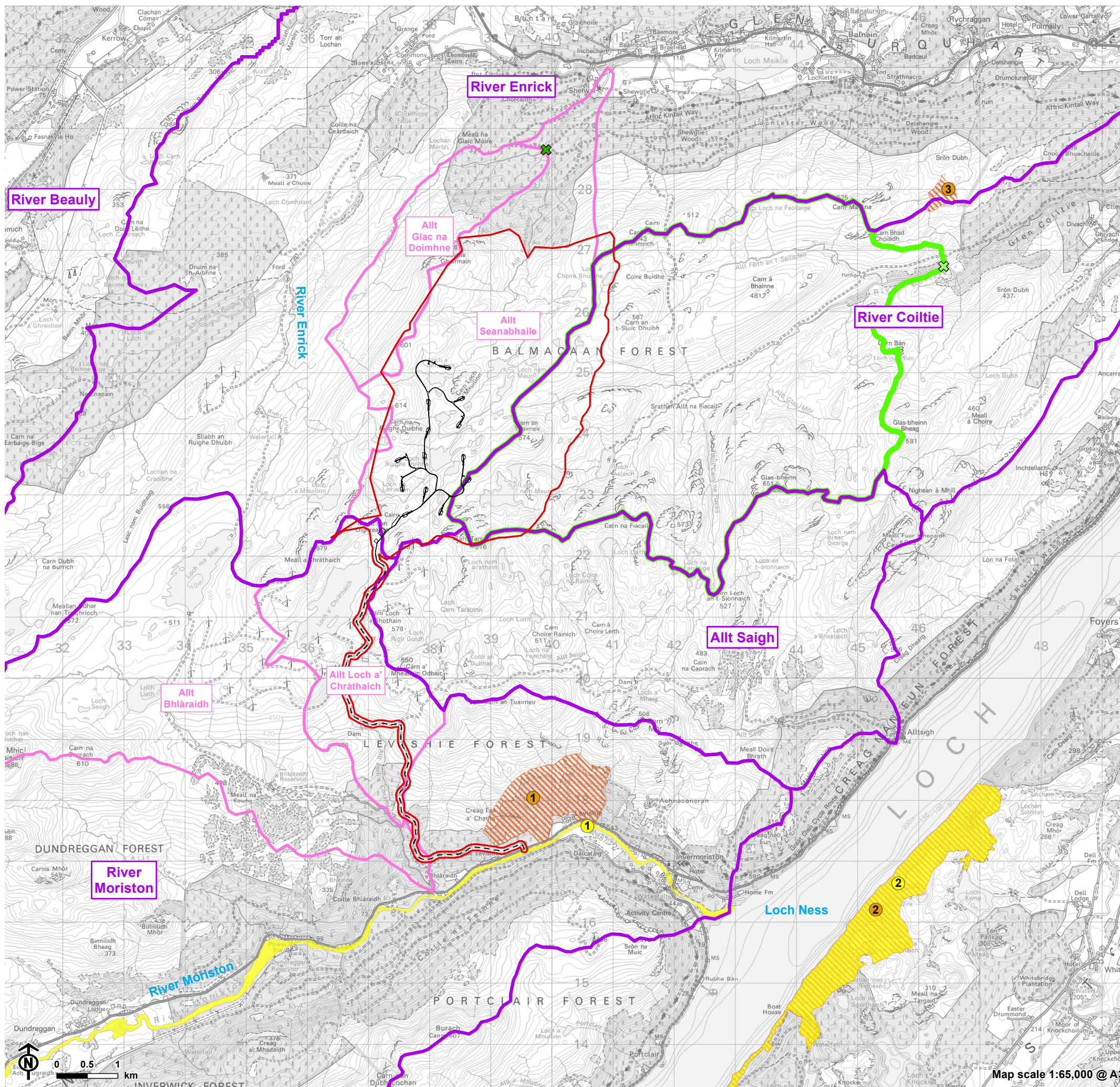
Figure 7.1: Hydrological Setting
