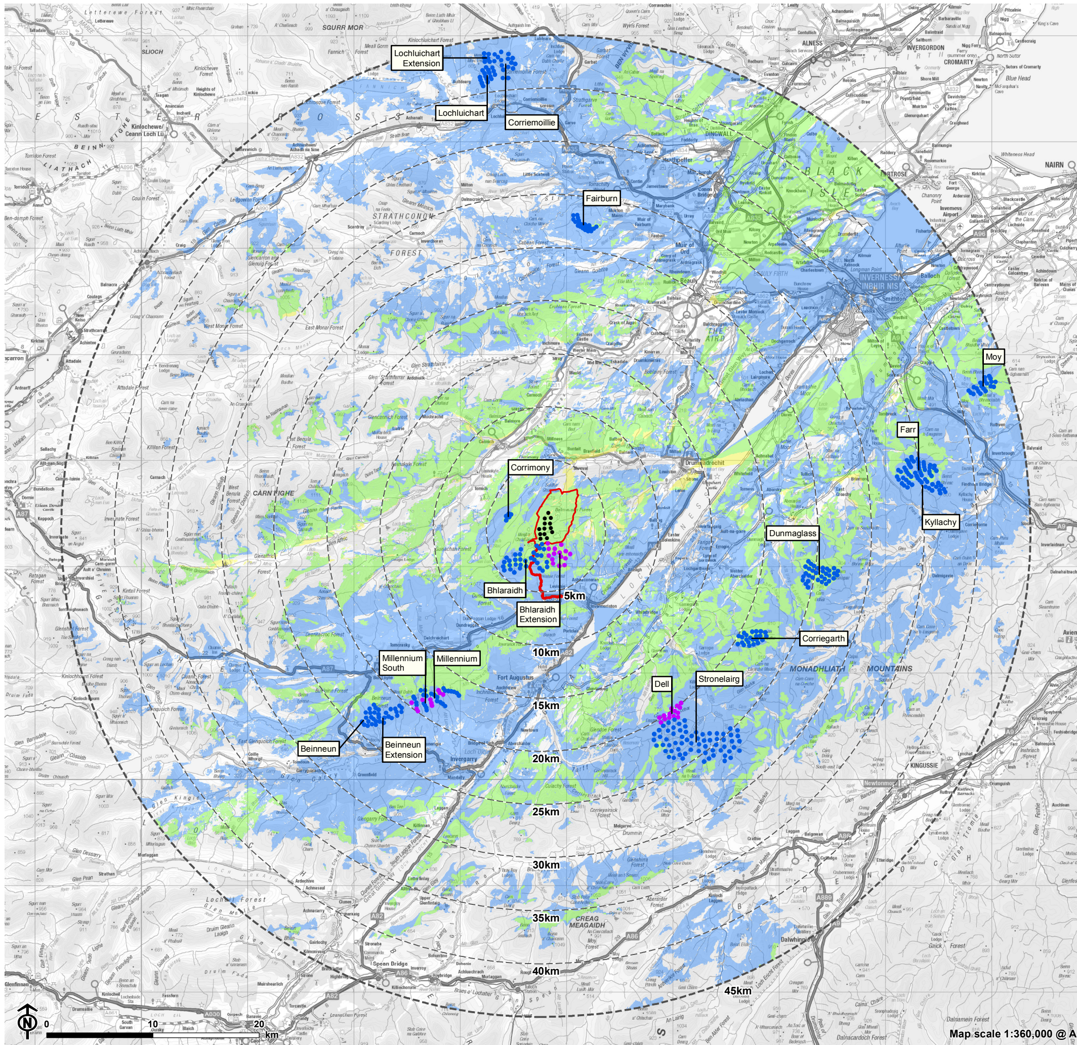
Figure 6.9: CZTV - Operational and Consented Wind Farms and Loch Liath
