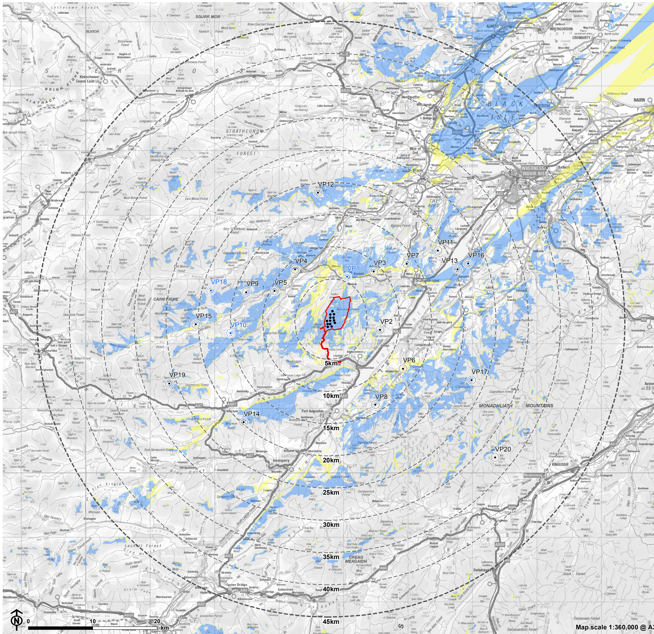
Figure 6.4: Blade Tip Height (180-200m) and Hub Height (102.5-122.5m) Comparative Zone of Theoretical Visibility (ZTV) and Viewpoint Locations
