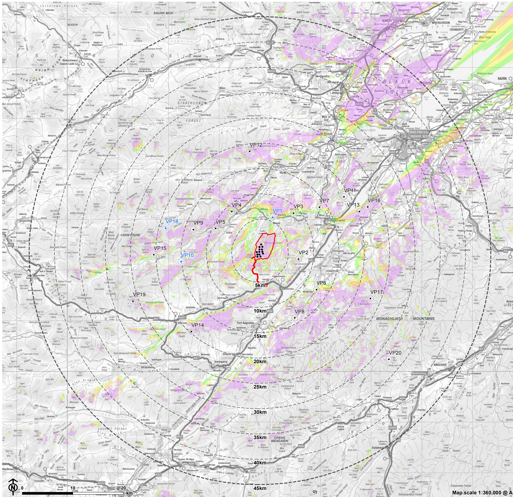
Figure 6.2a: Blade Tip Height (180-200m) Zone of Theoretical Visibility (ZTV) and Viewpoint Locations
