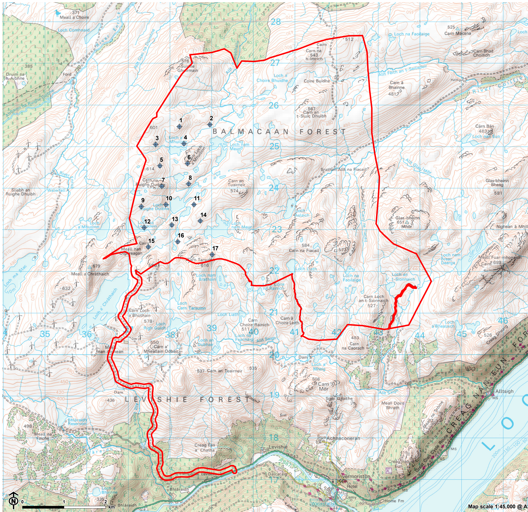
Figure 3.1d: Layout 4: 17 Turbines up to 200m to Blade Tip (this layout was presented to NatureScot and THC in November 2021)
