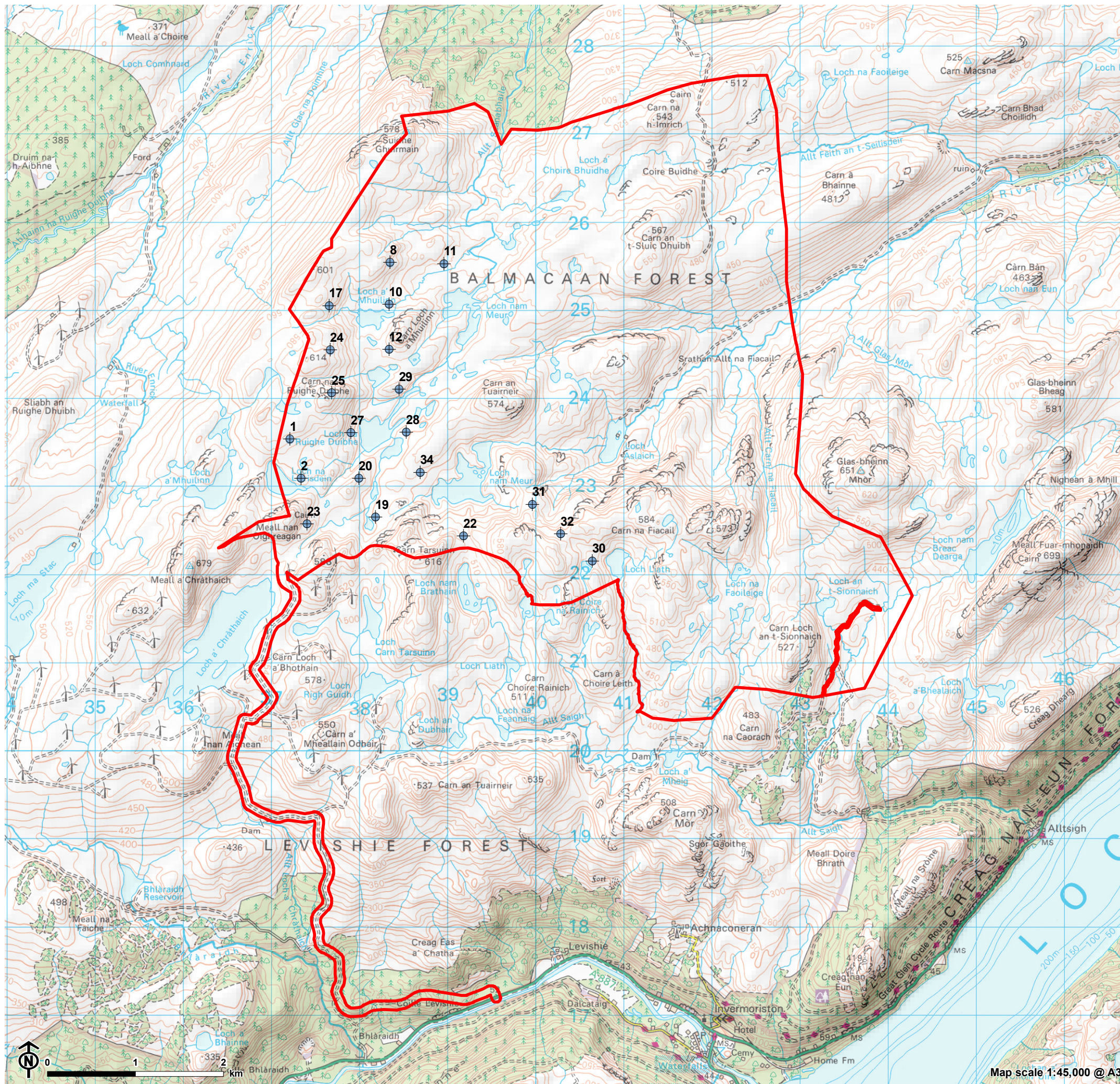
Figure 3.1c: Layout 3: 20 Turbines up to 200m to Blade Tip
