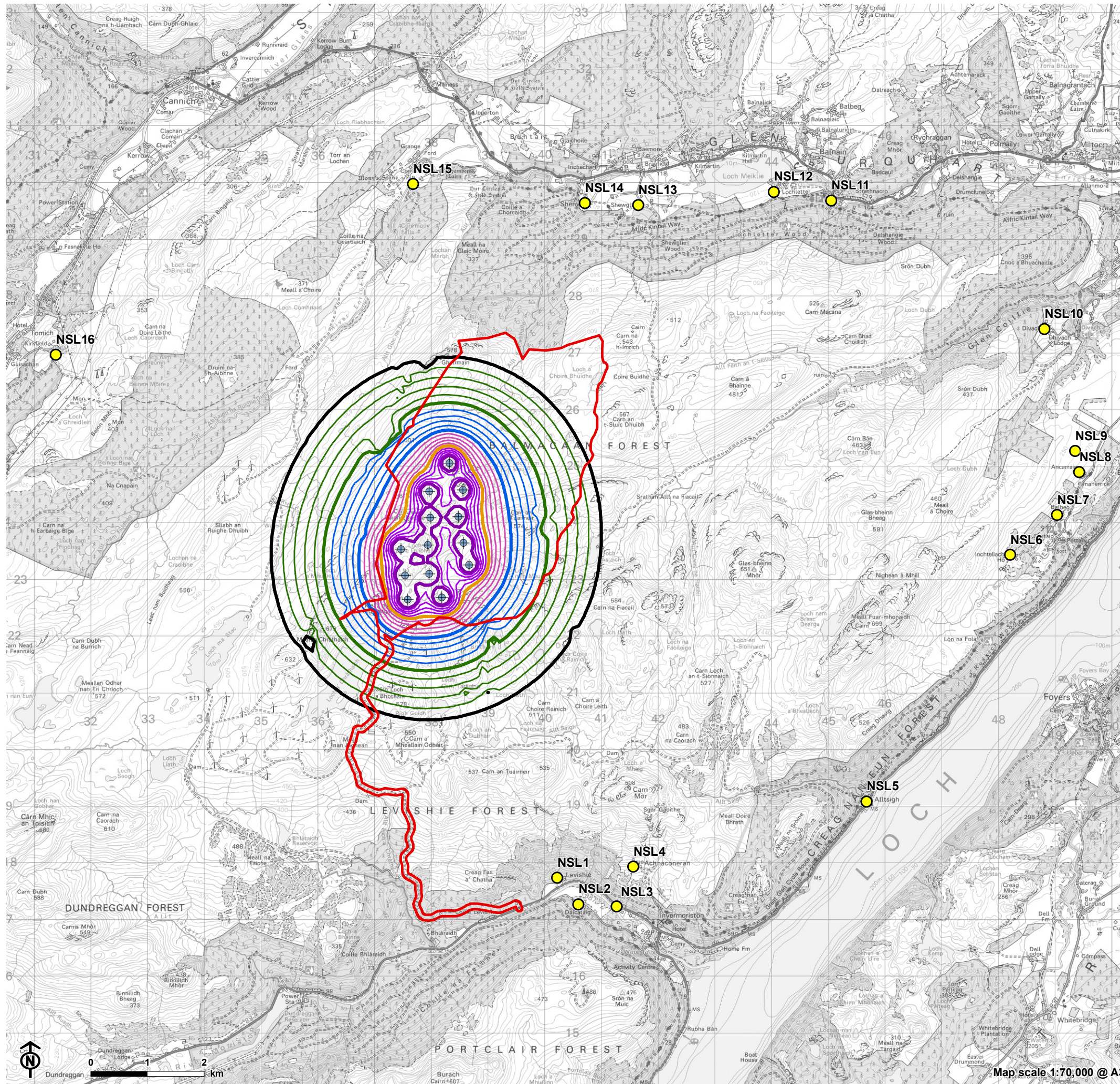
Figure 11.1: Noise Locations and Noise Contours
