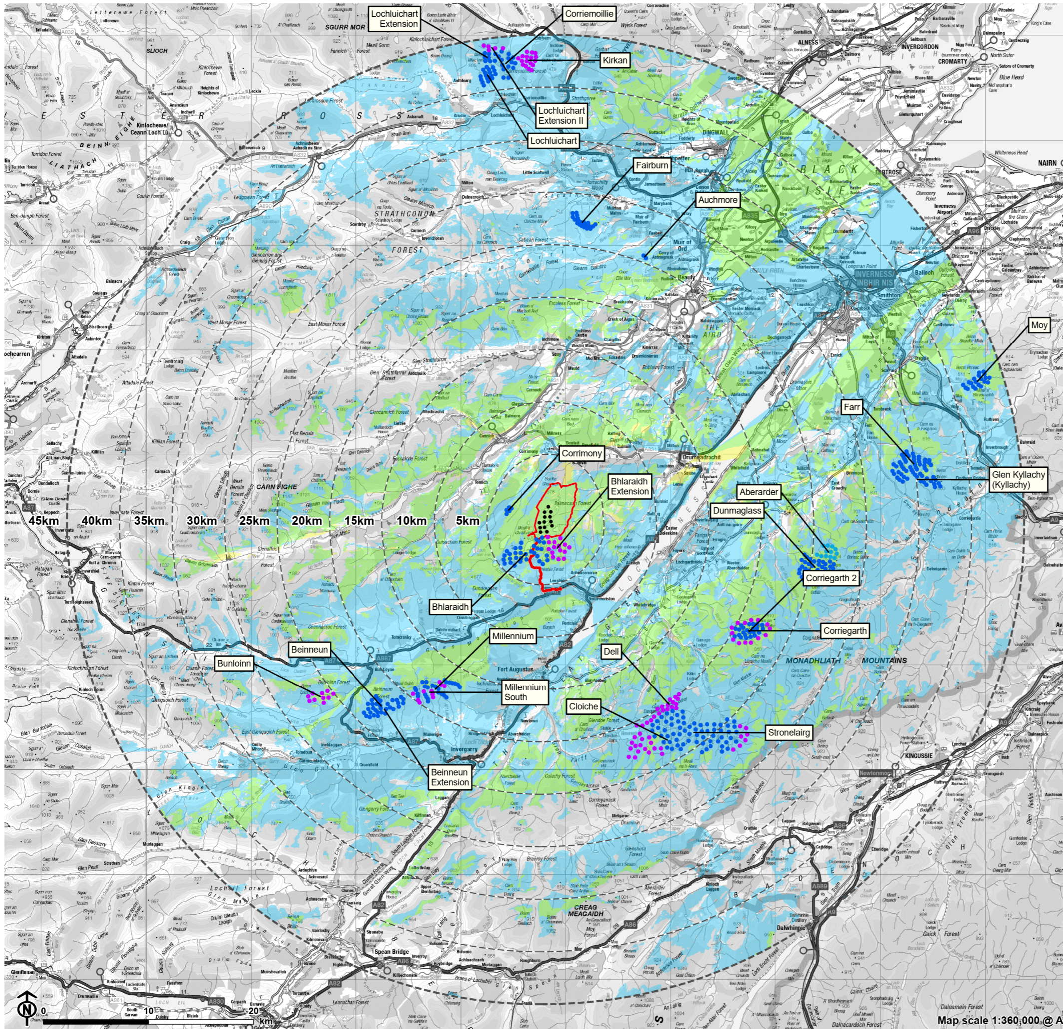
SEI Figure 6.9: CZTV – Operational, Under Construction and Consented Wind Farms and Loch Liath
