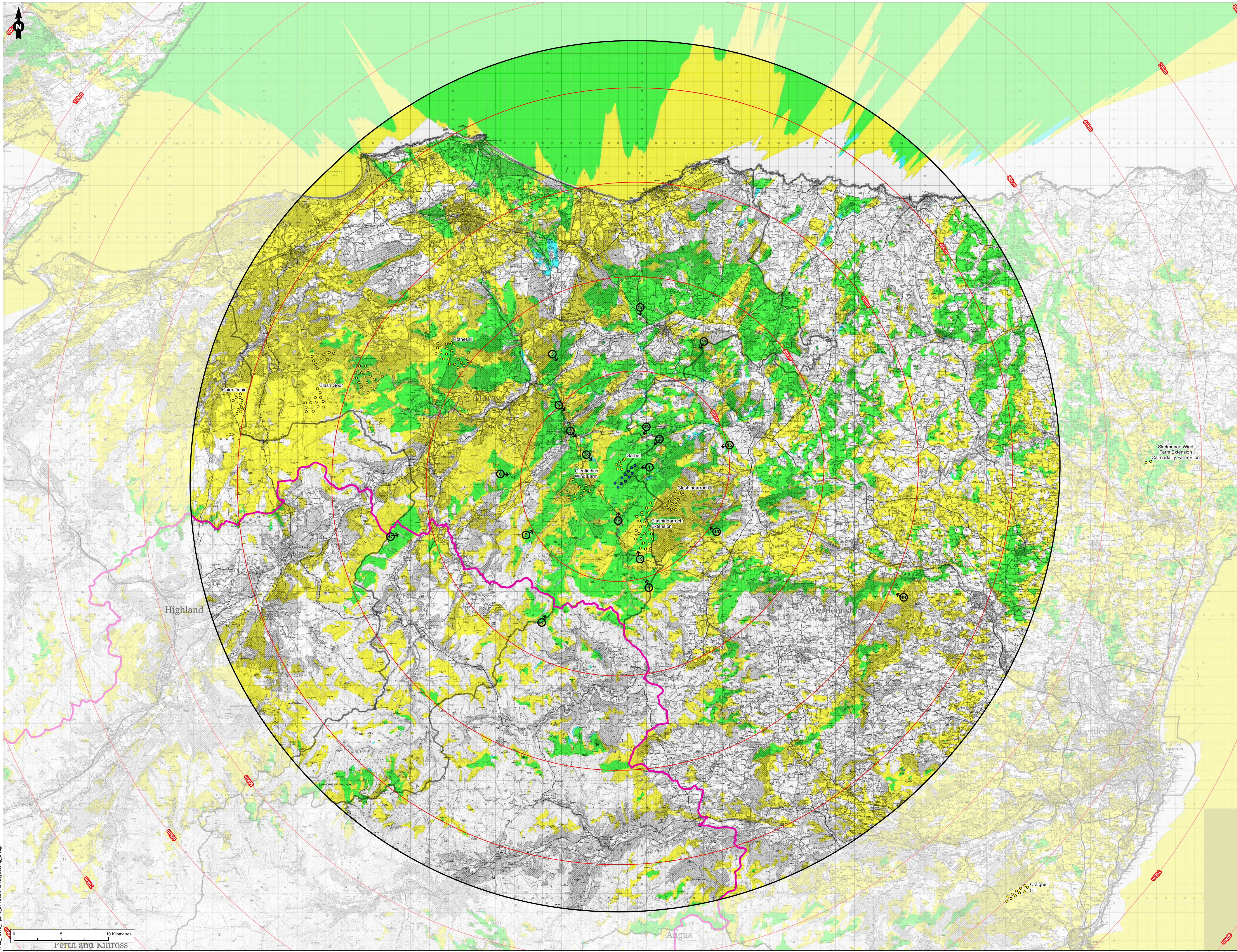
Figure Title Figure 5.7c: Blade tip/hub height ZTV comparison
