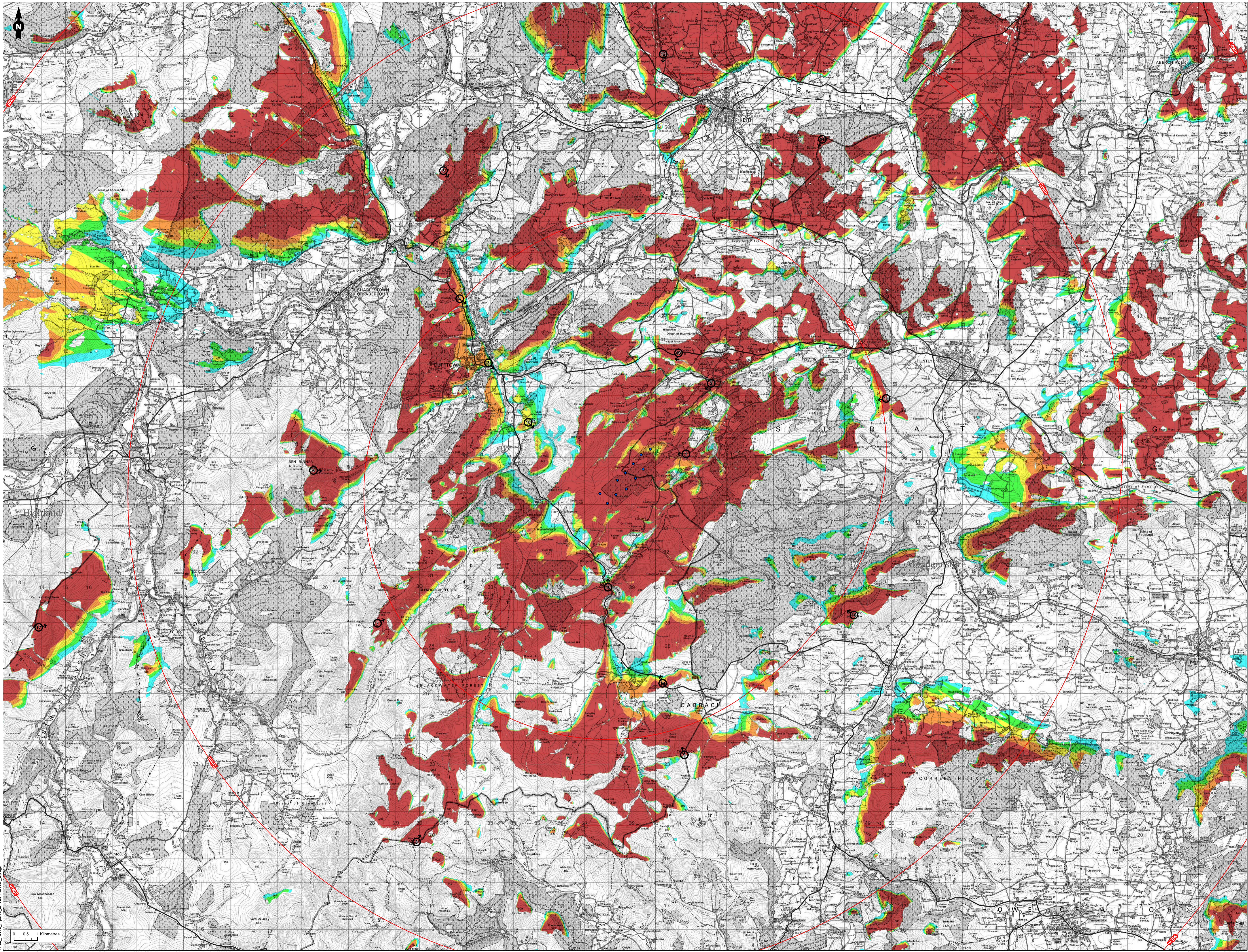
Figure Title Figure 5.6b: Blade Tip ZTV (20km Zoom)
