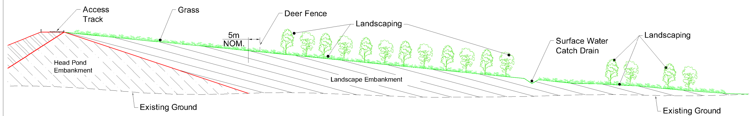
HEAD POND - INDICATIVE SECTION THROUGH LANDSCAPE EMBANKMENT - LOOKING WEST 1:500
