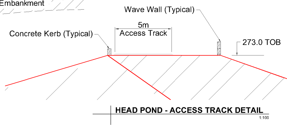
HEAD POND - INDICATIVE SECTION THROUGH LANDSCAPE EMBANKMENT - LOOKING NORTH 1:500
