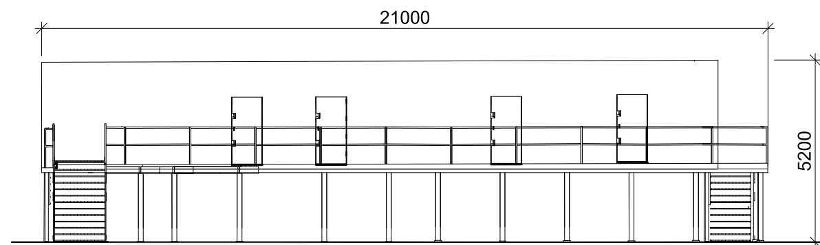
WEST ELEVATION
