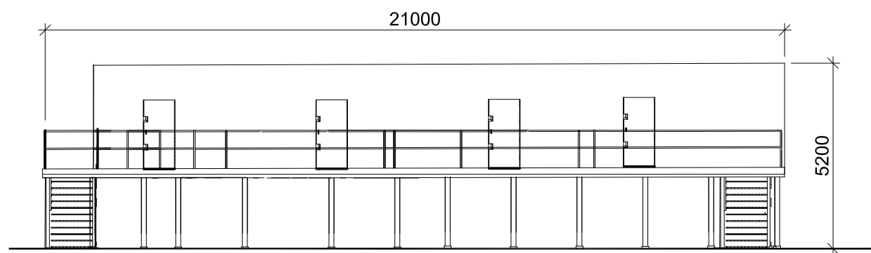
EAST ELEVATION
