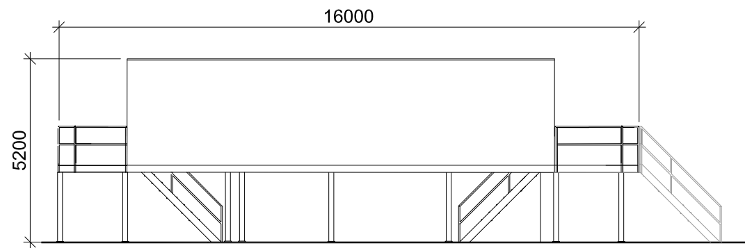
NORTH ELEVATION
