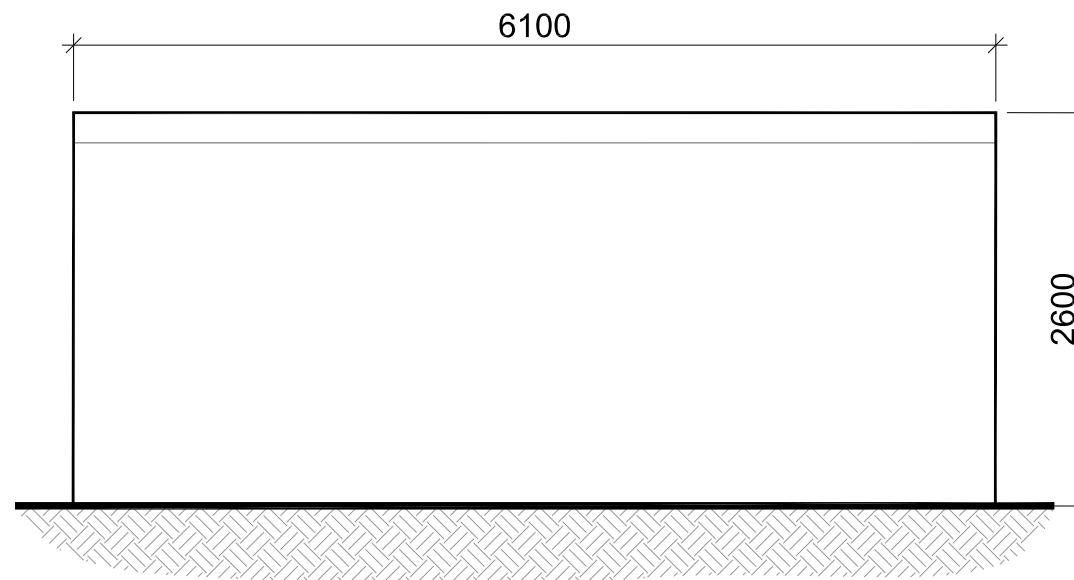
SOUTH ELEVATION
